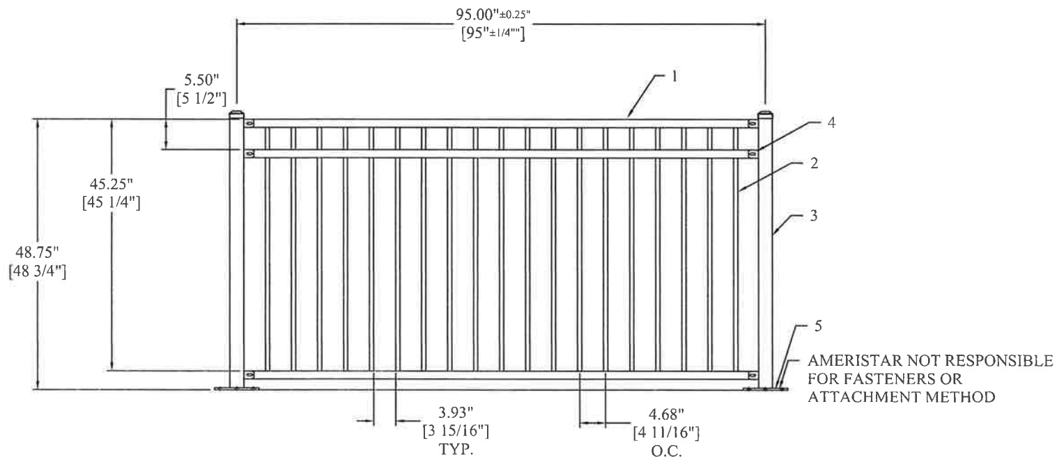
ELEVATION VIEW
